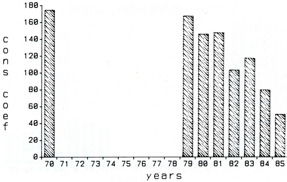
Fig. 6 — Evolution of the inbreeding coefficient in the Azores Archipelago from 1979 to 1985 and also in 1970. ( \infty \times 10^5 is the mean of the values of the all islands)
