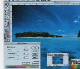
software
